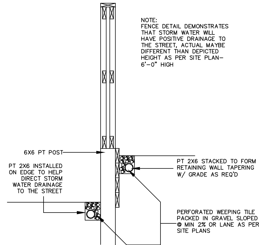
FENCE SECTION DETAIL
